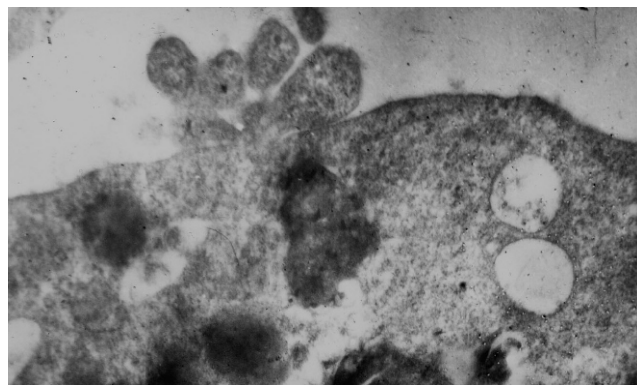
Fig. 3. Electronogram of MT-4 cells infected with HCV ( \times 15,000 )
